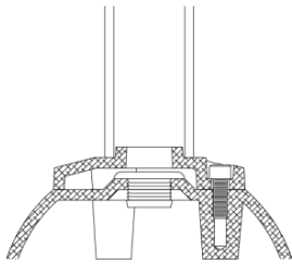
P3 - Pendant Small (3-Bolt Tenon Adaptor)
