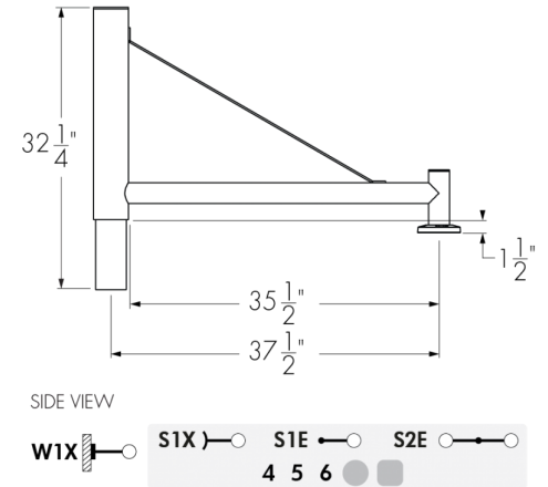
CS13 Arm Style
