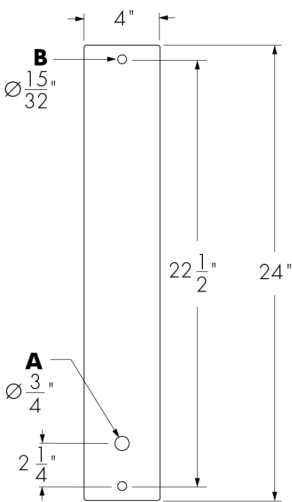
CS13 Arm Style Mounting Plate
