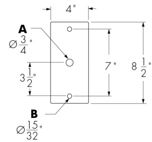
CS2 and CS12 Arm Style Mounting Plate
