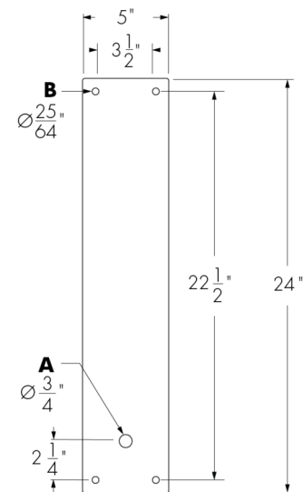
CS13 Arm Style Mounting Plate
