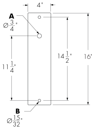
MC5 Arm Style Mounting Plate
