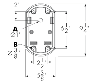
CS2 and CS12 Arm Style Mounting Plate
