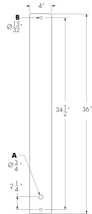
CS2 and CS12 Arm Style Mounting Plate
