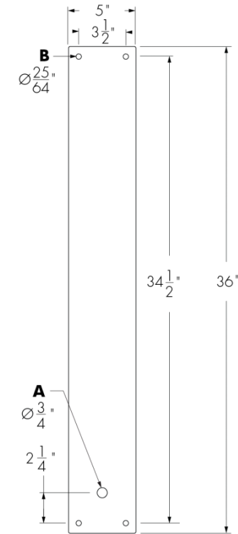
CS2 and CS12 Arm Style Mounting Plate
