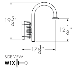
CS2 Arm Style
